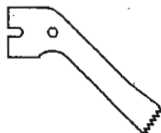
200-007 .25x4.1x15.0 mm
