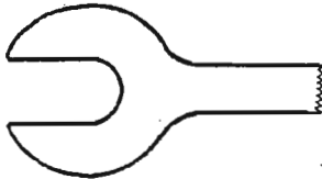
446-618 .4x5.5x18.5 mm
