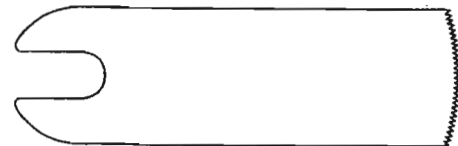
446-941 .4x19.0x41.0 mm
