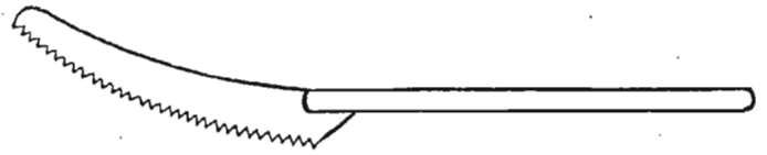
640-038 .6x6.0x40.0 mm
